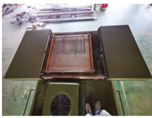
Charging pad on mining cars for sample delivery drones
